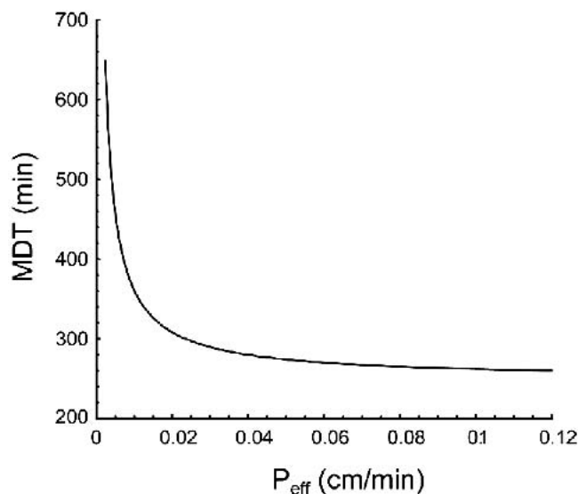
Fig. 3. The mean dissolution time ( MDT ) in the intestines as a function of P_{\text{eff}} for parameter values: M_0 = 10 mg, (1/q) = 0.2 , and r_0 = 10 \mu\text{m} . MDT is calculated as the area under the curve of the undissolved fraction of dose using the integral, MDT = \int_0^{\infty} (r_p/r_0)^2 dt in conjunction with Eqs. 5 and 6.
