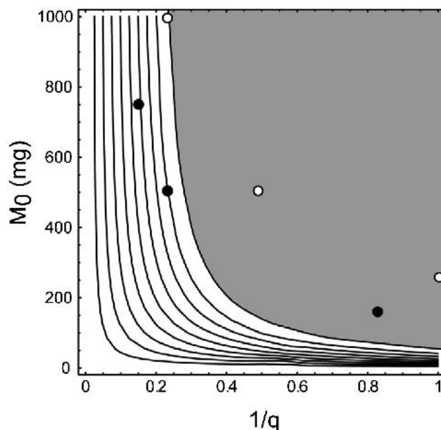
Fig. 2. Plot of dose, M_0 , versus the dimensionless solubility/dose ratio, 1/q . The curves indicate stepwise increase of 10% of absorption from left to right (range 10–90%) for parameter values r_0 = 25 \mu\text{m} and P_{\text{eff}} = 1.2 \times 10^{-2} cm/min. The open circles denote a drug administered in doses 250, 500, 1000 mg with solubility 1 mg/ml while the black dots denote a drug administered in doses 150, 500, 750 mg with solubility 0.5 mg/ml. Drugs located in the shaded region are fully absorbed ( F > 0.90 ) Class II drugs.
